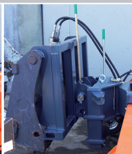
Roller floating tunnel with height indication and pendulum adapter
